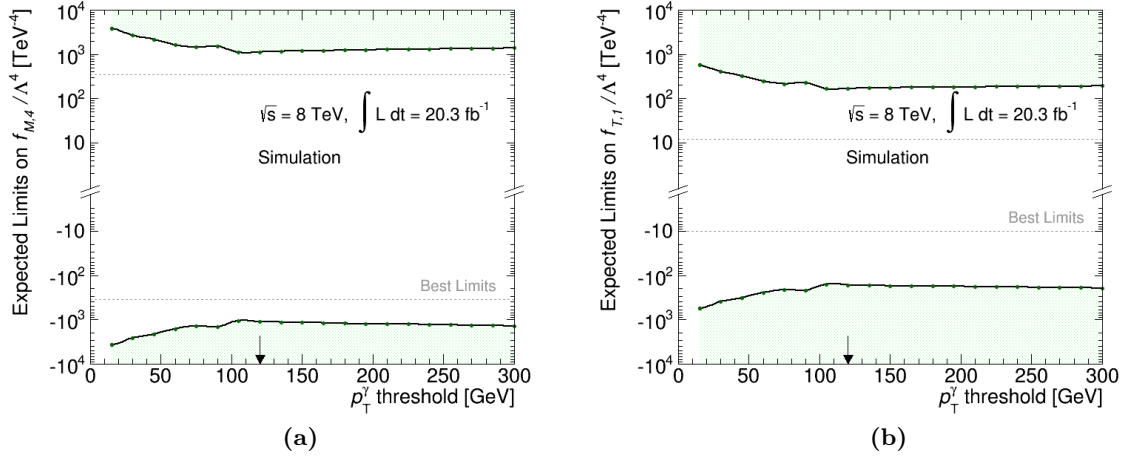
Figure 8.5: Expected limits at 95 % confidence level on f_{M,4}/\Lambda^4 (a) and f_{T,1}/\Lambda^4 (right) as function of the photon p_T threshold of the event selection. The coloured area corresponds to the excluded values of the corresponding coupling. Also indicated are the current best limits from References [23] (b) and References [24] (right). The optimal p_T^\gamma threshold, chosen for stability reasons to correspond to 120 GeV, is shown by the arrow.
