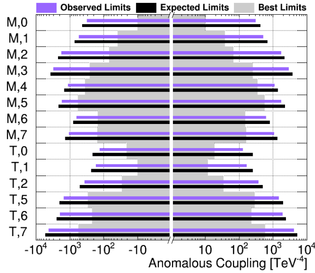
Figure 8.6: Visualisation of the observed and expected limits at 95 % confidence level on the different anomalous quartic gauge couplings. The current best limits are shown in grey and come from different analyses [23, 24, 110, 111] as detailed in Table 8.2. For brevity, only the index i of the coupling f_i/\Lambda^4 is indicated in the figure.
